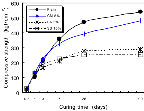
Fig.3 Compressive strength of mortar according to accelerator type
