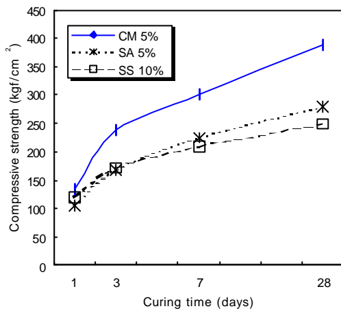
(a) Compressive strength
