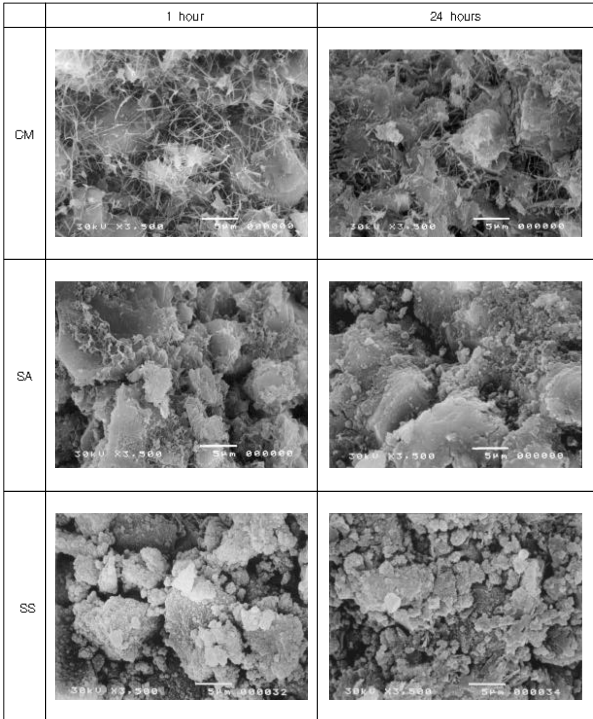
Fig.6 SEM photographs according to accelerator type
