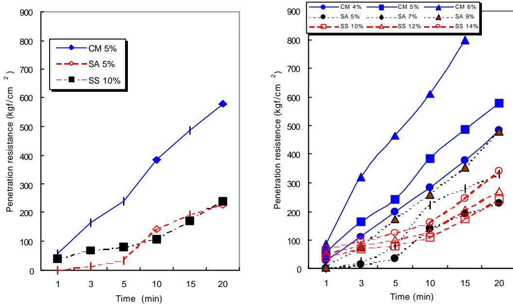
Fig.1 Proctor penetration resistance of mortar according to accelerator type
