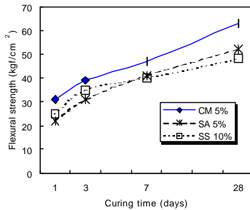
Fig.5 Flexural strength of concrete according to accelerator type (10×10×35cm Beam type specimen)
